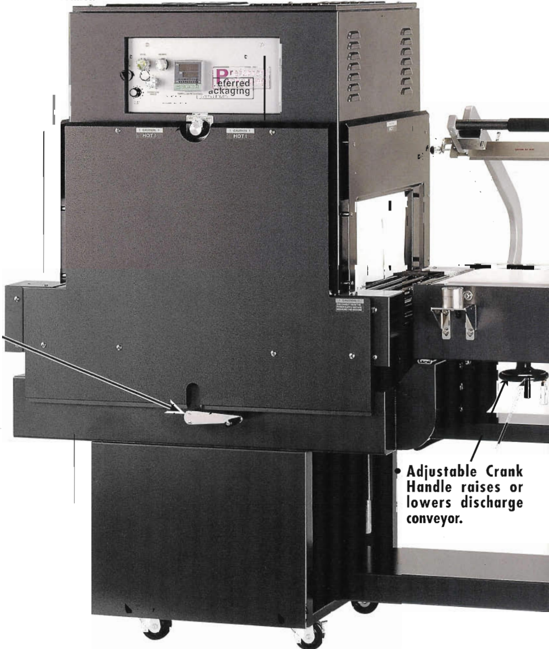
Linear bearings allow sealer to easily move forward or backward to center package into tunnel.
